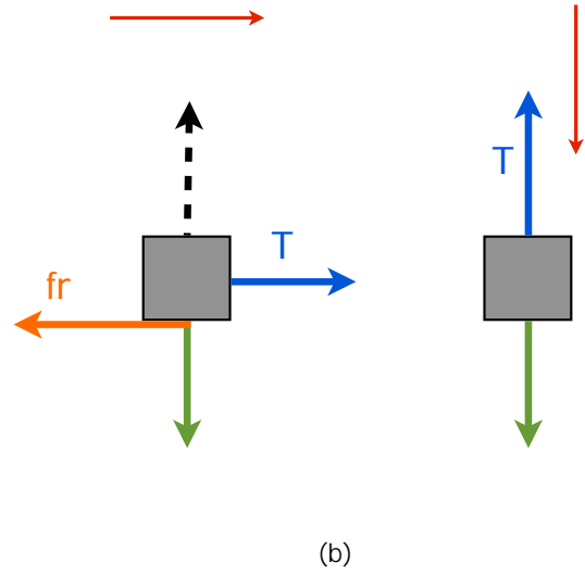
Figure 2: (a) Pulley system used to calculate u_k . (b) Free body diagrams for the pulley setup. W_i is the weight of the object and fr is the frictional force.
